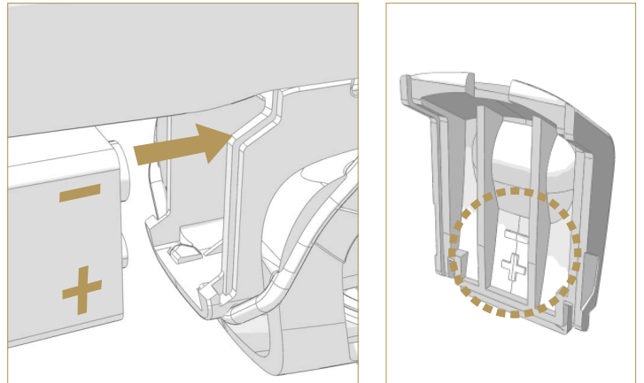
Insert the battery with the negative terminal on top
