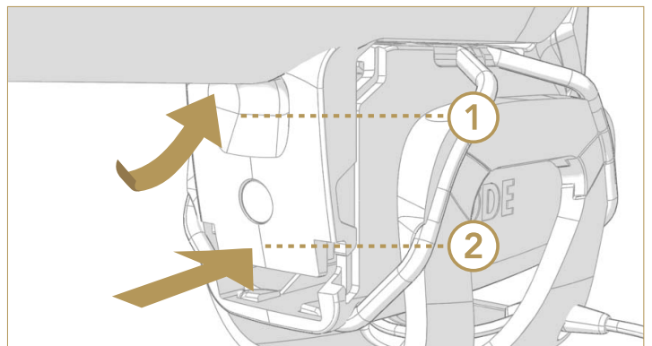
Push up on the indentation with your index finger then pivot the bottom of the cover away
